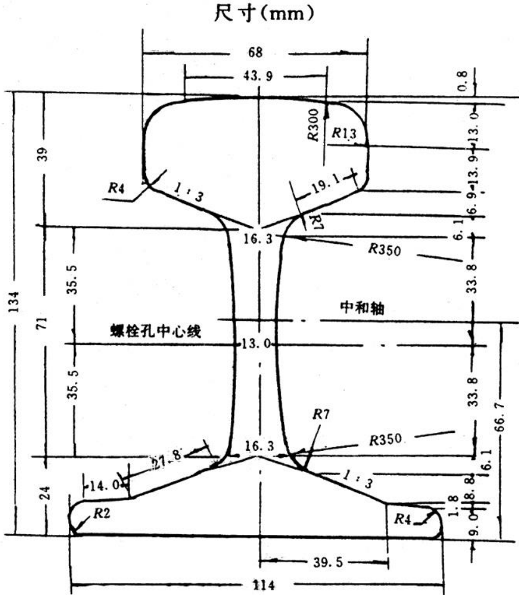
38kg/m railway rail
